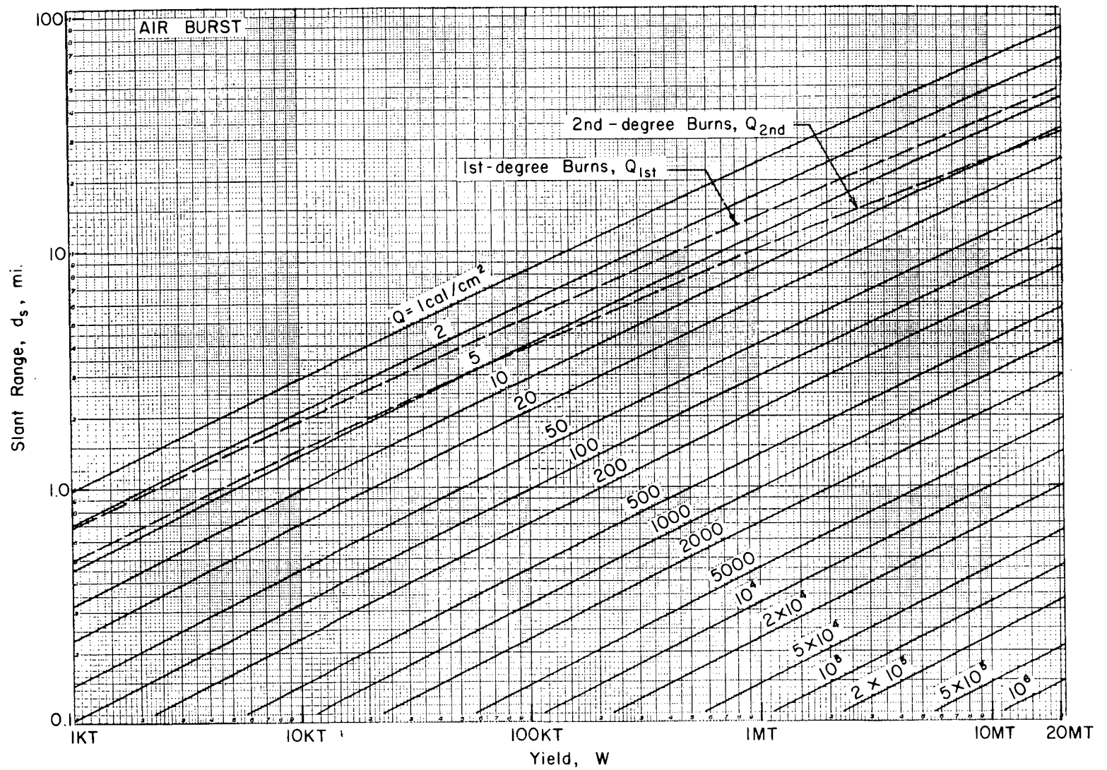
Fig. 2.12—Thermal radiation for air bursts as a function of yield and slant range (50-mile visibility). Also shown are first- and second-degree-burn lines applying to bare white skin as a function of yield (see Eqs. 2.108, 2.110, and 2.111 in Table 2.11).
